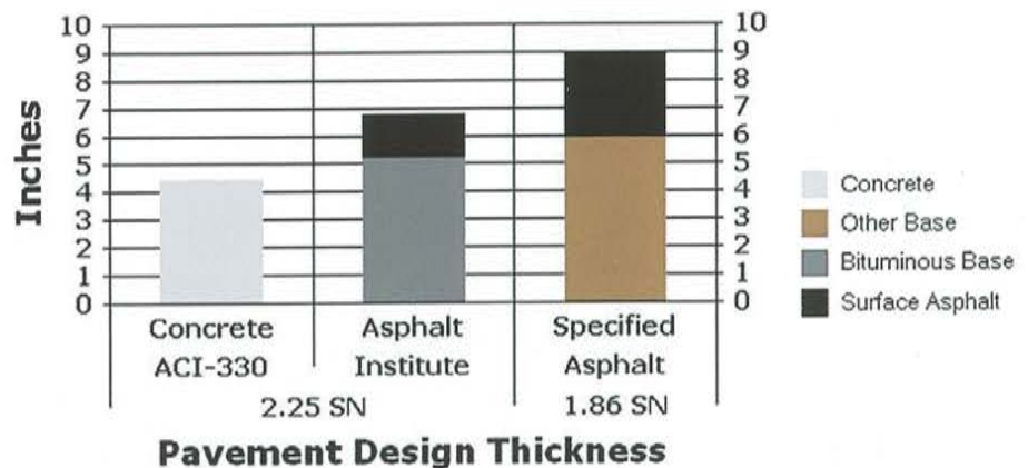
Design Summary - Parking Area
